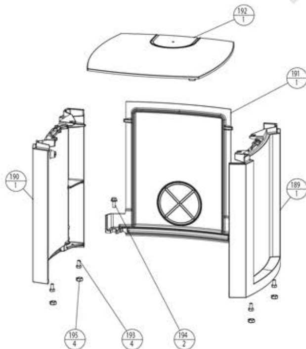
351205 Cast Iron Base Jøtul F274 BP 351206 Cast Iron Base Jøtul F274 GP
