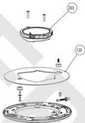
350997 Revolving pedestal Jotul F 270 / F370
