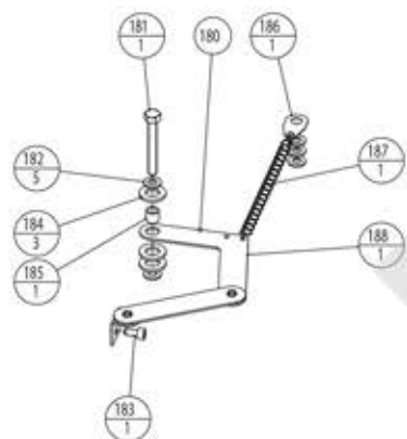
351113 Self Closing Mechanism Jotul F 270
