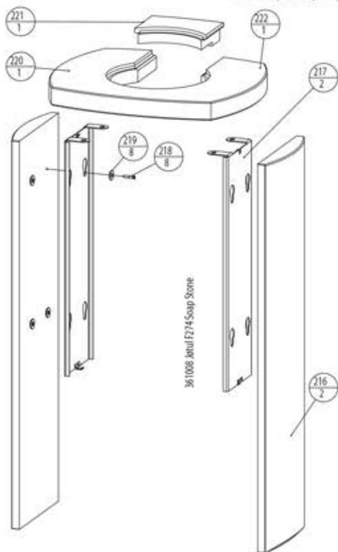
361009 Soapstone Top Complete Jotul F 270
