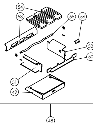
Optional Wood Ash Removal Kit
