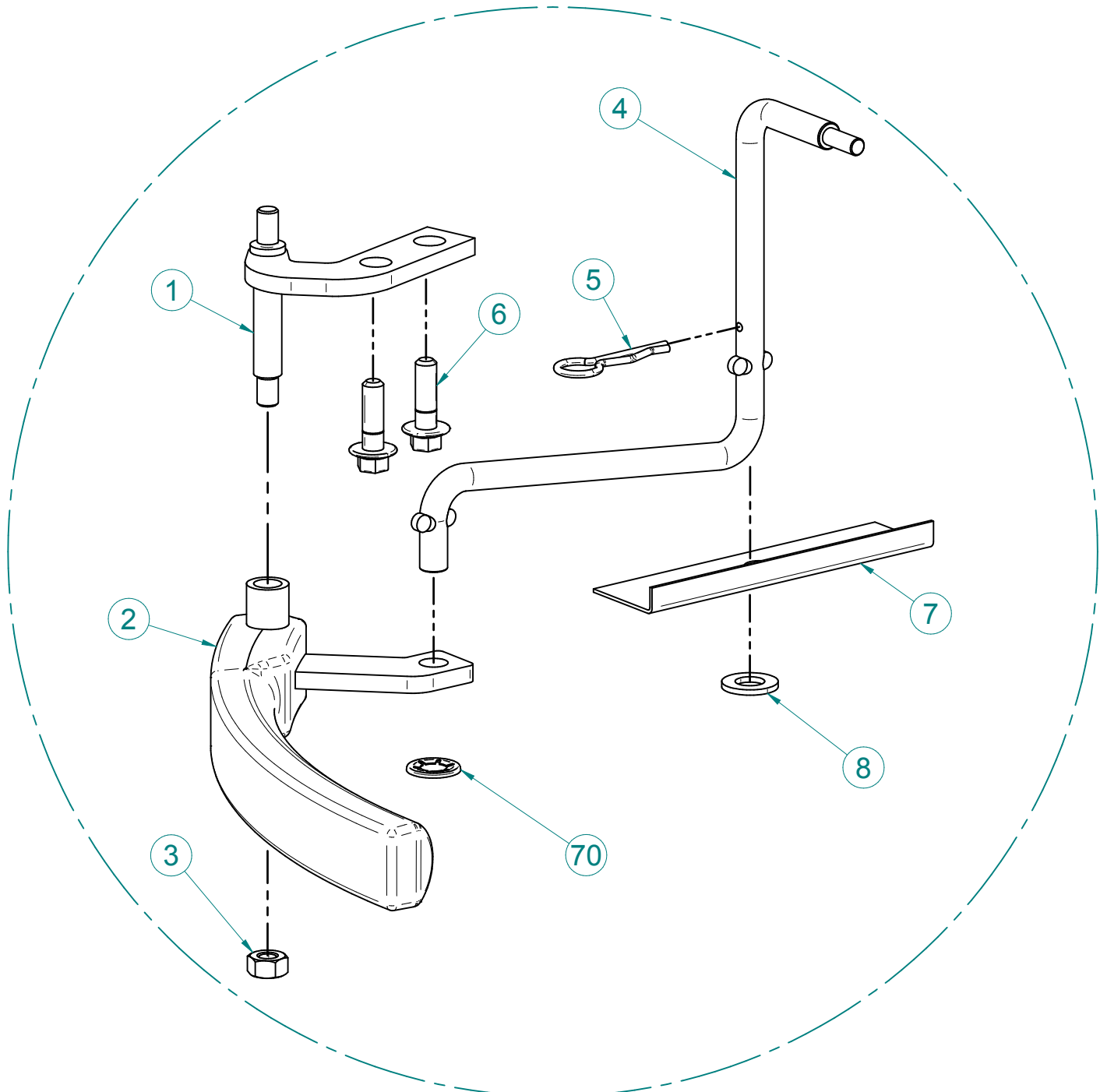
DETAIL A
